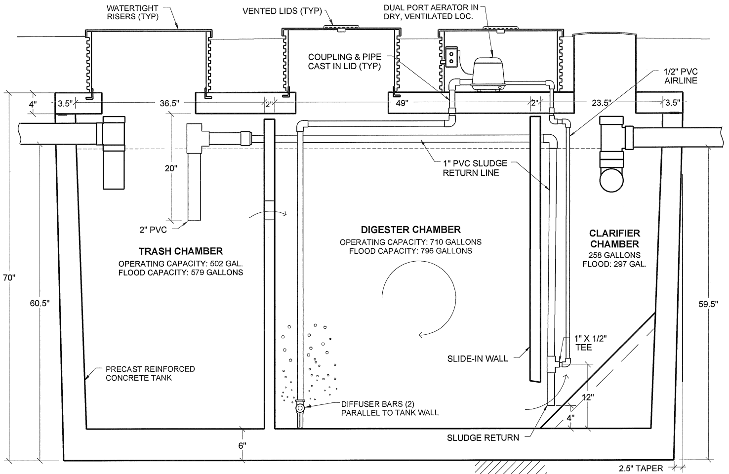
BNR-750 SIDE VIEW NO SCALE
