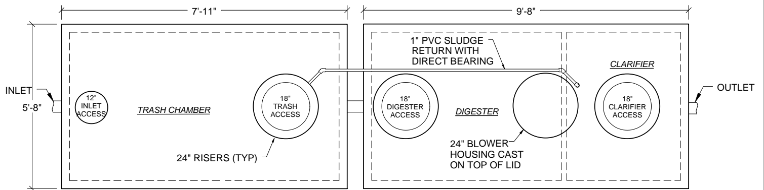
BNR-1000 TOP VIEW NO SCALE
