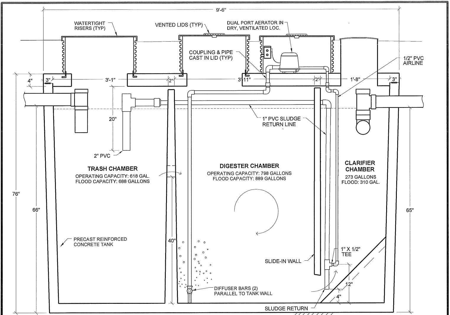
BNR-750 SIDE VIEW NO SCALE
