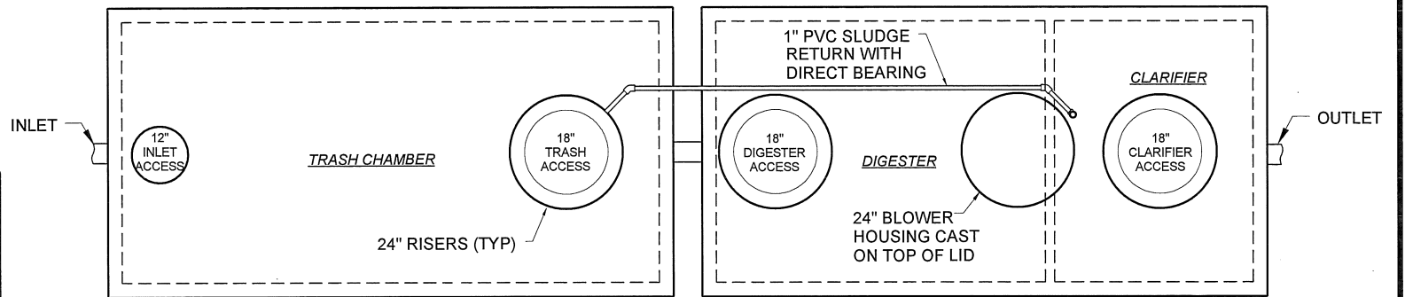
BNR-1500 TOP VIEW NO SCALE
